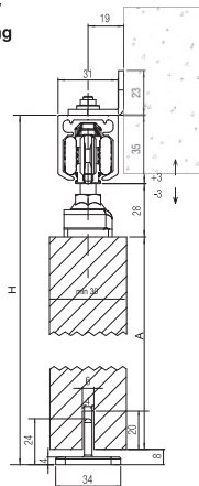
Section View Wall Mounting
