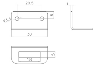
Strike Plate
