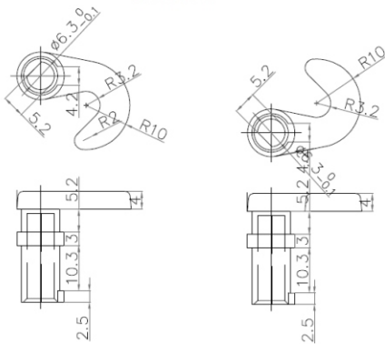
Lock Hook
